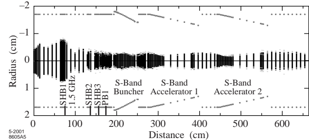
Figure 4. The beam envelope in the injector, based on simulations with PARMELA
