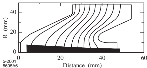
Figure 2. CTF3 gun ray trace from EGUN. 5 A, 140 kV grid limited mode.
