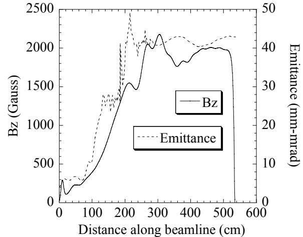
Figure 3. The longitudinal magnetic field and the beam transverse, normalized, rms emittance along the CTF3 injector. X = 0 is at the anode tip.
