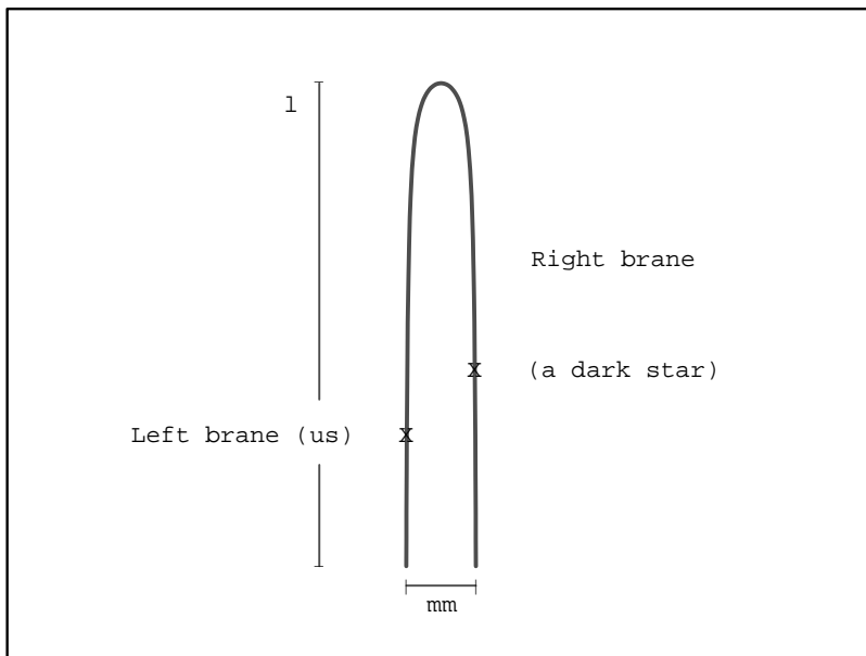
Figure 1: The Bifold universe. The distinction of matter between the Standard Model particles on the left-brane and the dark particles on the right-brane is not microphysical but purely geometrical.
