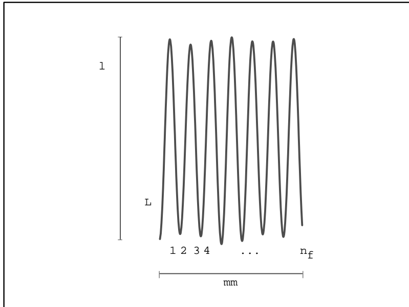
Figure 2: The Manyfold universe. Each side is referred to as a brane, or a fold, while the region where they connect is called a tip of a fold. We live on the leftmost brane L , while there are n_f right-branes in the bulk adjacent to our brane.
